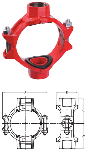
Mechanical Cross Threaded Outlet
